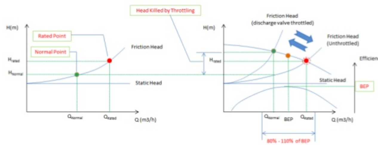
Fig-6: Pump Selection at Rated flow, BEP between Normal and Rated
