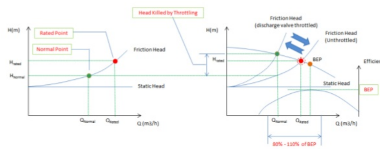
Fig-7: Pump Selection at Rated flow, BEP is NOT between Normal and Rated
